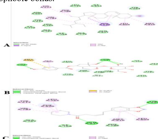
Figure 1. Protein-Ligand Interactions of the three best docking results of 70% ethanol extract samples of the pericarpium of the Kunto Bimo fruit ( Kigelia africana (Lam.) Benth.) (A) Sitosterol (B) 7-hydroxy-7-methyl-1- \{[3,4,5\text{-trihydroxy-6-(hydroxymethyl)oxan-2-y}
