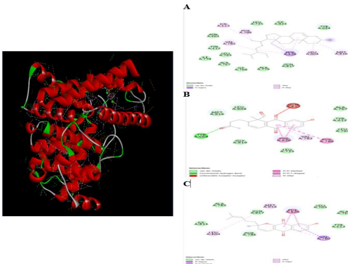
Figure 3. Protein-Ligand Interactions of the three best docking results of 70% ethanol extract samples of semen from the fruit of Kunto Bimo ( Kigelia africana (Lam.) Benth.) (A) Sitosterol (B) Sterekunthal A (C) (2s)-8-hydroxy-2-methyl-2-(4-methylpent-3-en-1-yl)benzo[g]chromene-5,10-dione.
