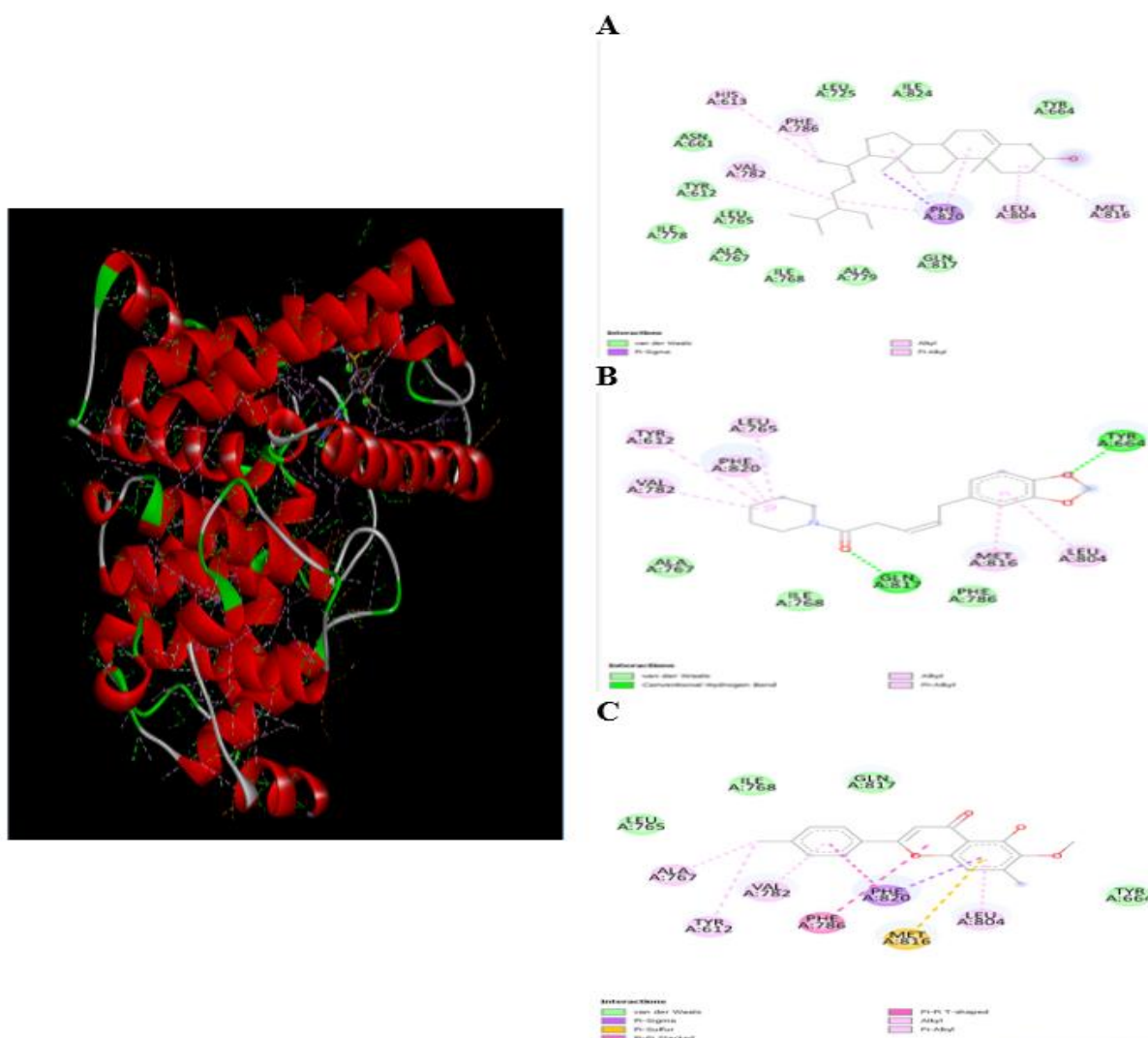
Figure 2. Protein-Ligand Interactions of the three best docking results of 70% ethanol extract samples of the fructus of the Kunto Bimo fruit ( Kigelia africana (Lam.) Benth.) (A) Sitosterol (B) Piperine (C) 5-hydroxy-6-methoxy-7-methyl-2-(4-methylphenyl)chromen-4
